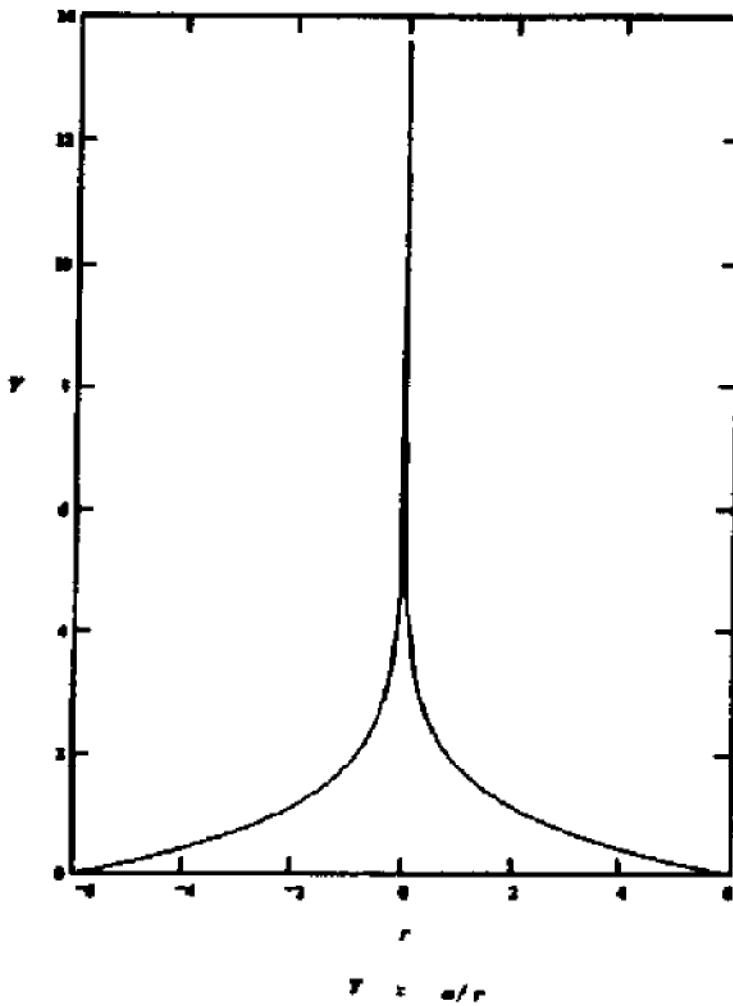
Coulomb Potential of Isolated Charged Particle
