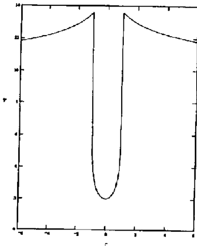
Coulomb Potential of Two Adjacent But Otherwise Isolated Particles
